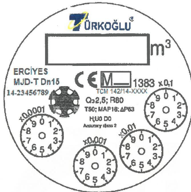
Figure 10: The dial plates of the water meter type ERCIYES MJD-xx-T with register 8+1:
